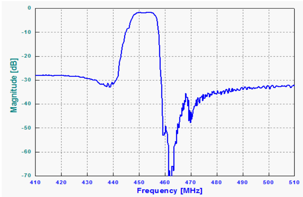
Frequency Response
